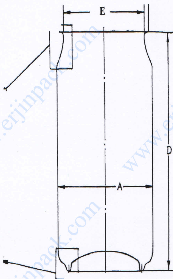
FINISHED CAN 成品罐
